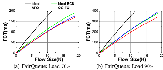
Figure 15: Average FCT comparisons under different flow size on W6 for Fair Queuing.
