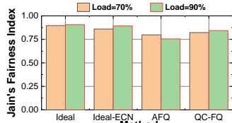
Figure 14: Jain’s Fairness Index of different Fair Queuing Algorithms on W6.
